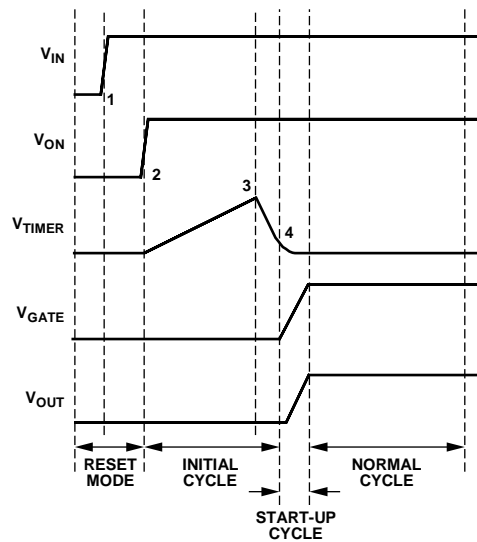
Figure 36. Power-Up Timing
