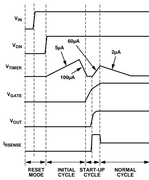
Figure 37. Power-Up into Capacitor
